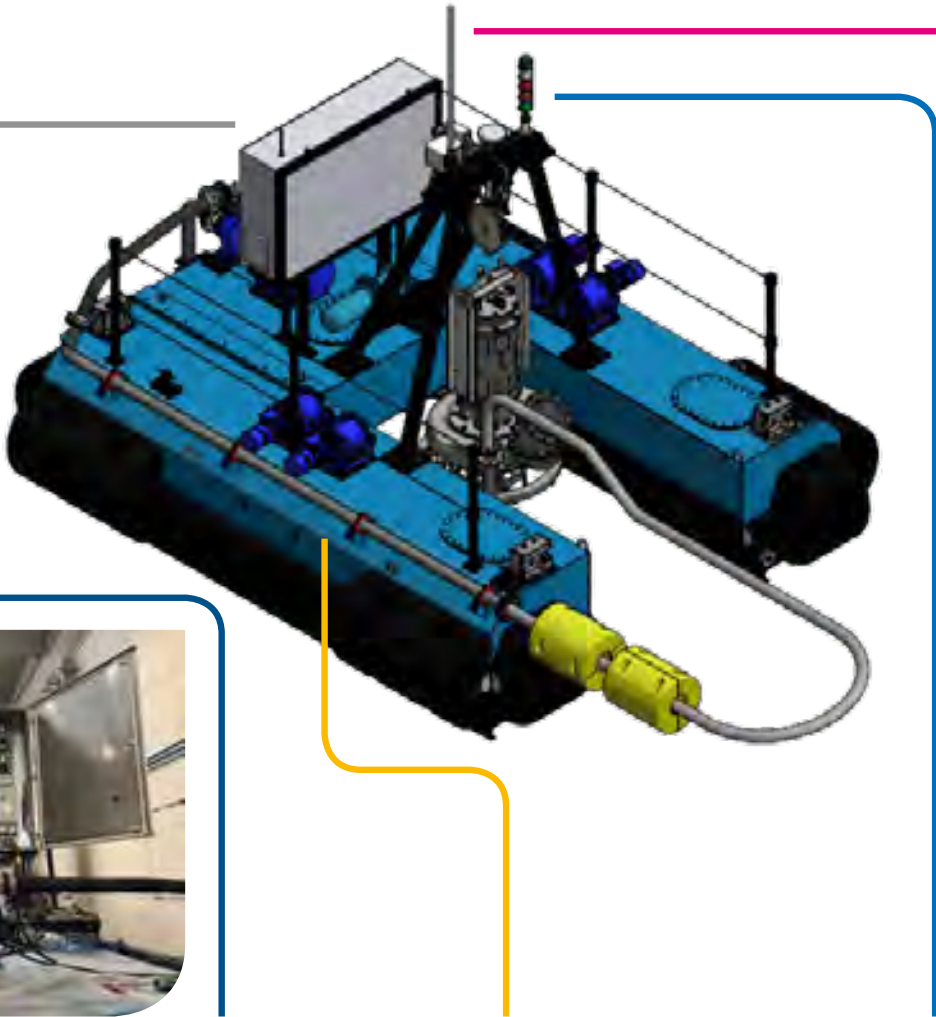
Cooling Jacket System
